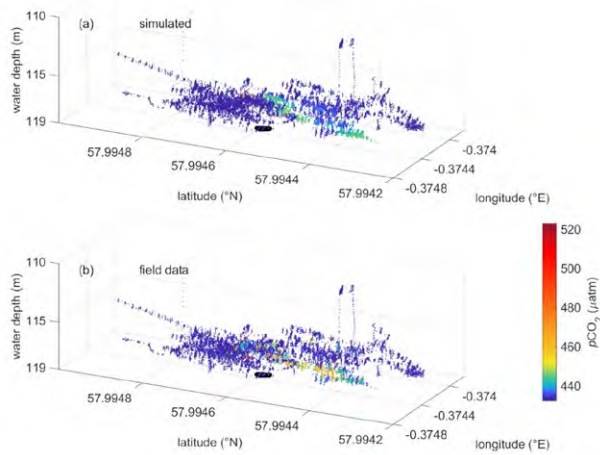
Fig. 3: Comparison of simulated (a) and measured (b) spatial distribution of p\text{CO}_2 in the water column during injection of 143 kg \text{CO}_2 per day into sediment at Goldeneye. The black shape indicates the bubble release site (Gros et al., 2021).
