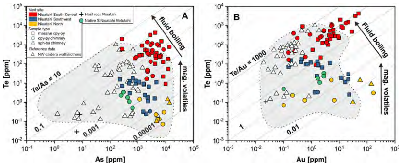
Fig. 2: In-situ LA-ICP-MS composition of hydrothermal pyrite compared to the composition of the magmatic host rock (this study), native S from Niutahi Motutahi (Kim et al. 2011) and pyrite from other subduction zone-related systems (Keith et al. 2016).
