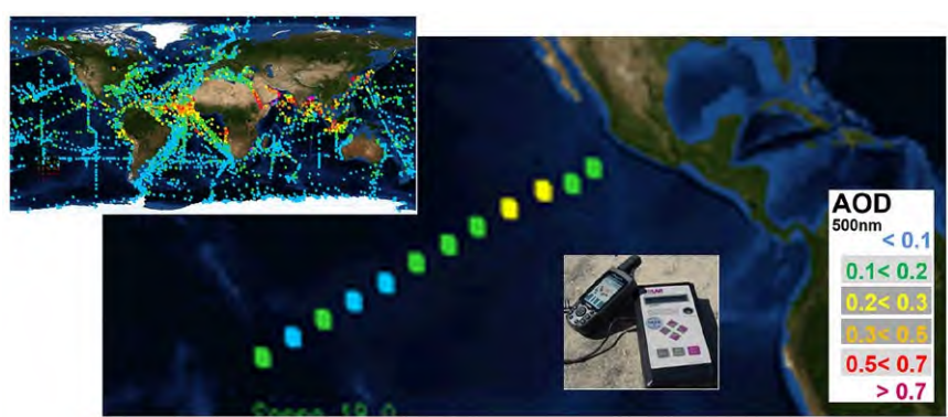
Fig. 1: daily AOD averages during the SO267/2 cruise in the context off all shipborne samples contributed to the MAN data-base over the last 18 years (left, upper corner).
