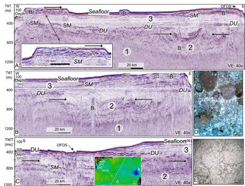
Fig. 2: Seismic profiles of SMB (Position in Fig. 1B) with clinoform progradations (arrows) and drowning unconformity DU. A: W-E line. B: Carbonate banks, SM: sea-floor multiple. Inlay: Detail showing progradation in carbonate body. OFOS: image shown in D. B: Eastern part of W-E line. C: SSW-NNE line with DU hardground and sediment cover thickening towards the north. OFOS: image shown in E. Inlay with multibeam imagery and path of seismic profile (stippled line); d: submarine dunes; k: karst collapse. D: MEC (water depth: 30 m) with corals and coralline red algae. Scale bar: 40 cm. E: DU hardground (water depth: 302 m). Scale bar: 40 cm. From Betzler et al. (2021).
