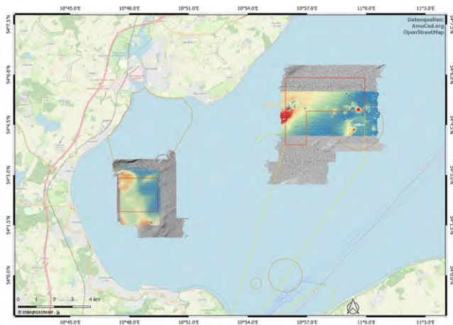
Fig. 1a: Lübeck Bay with bathymetric data acquired during POS530 (color) and data recorded in 2020 and 2021
