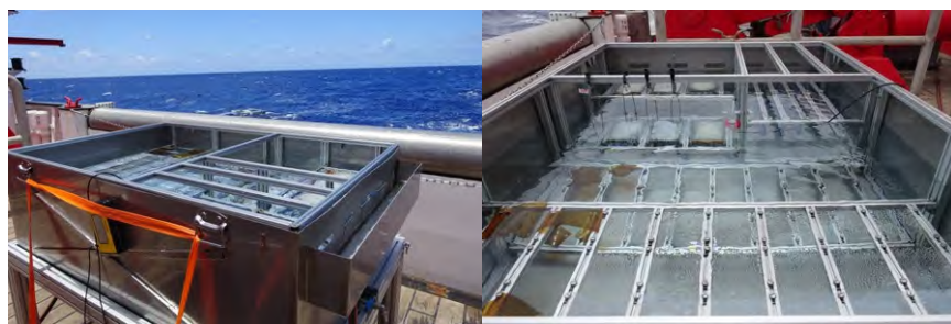
Fig. 1: View of one of the mesocosms installed on board the ship (left) and position of the samples: Sheets and PET bottles in the foreground, granules in nets in the background (right).
