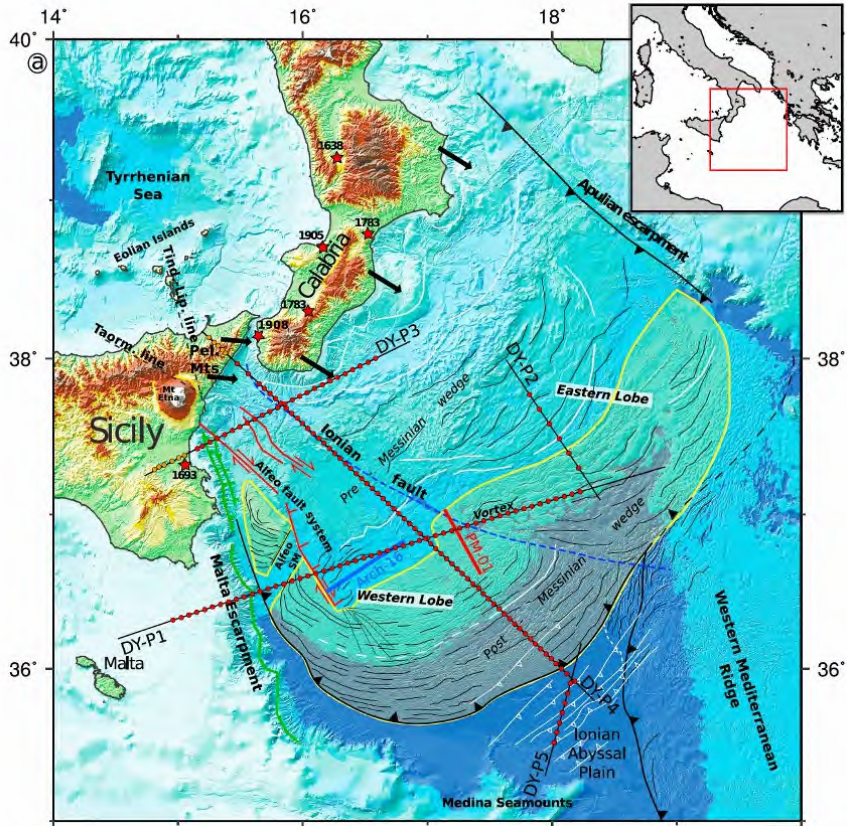
Fig. 1: Interpreted bathymetric map of the Ionian basin (Dellong et al., 2018; Gutscher et al., 2016). Superposed the wide-angle profiles from the M111 cruise (named DY-P1 through DY-P5) with small red dots for the ocean bottom seismometers and orange dots for the land-stations. The red stars show the positions of major earthquakes and their corresponding dates.
