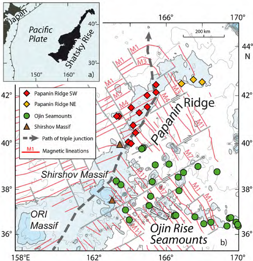
Fig. 1: a) Overview map of Shatsky Rise. b) Close-up map of Papanin Ridge emanating from the northern part of Shatsky Rise and the Ojin Rise Seamounts east of Shirshov Massif showing the sample locations of this study in different colors depending on their structural affiliation. Map modified after Sager et al. (2010) with magnetic anomaly lineations (red) after Nakanishi et al. (1999).
