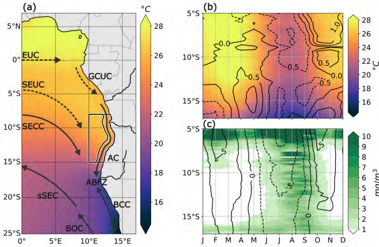
Fig.1: (a) Schematic circulation in the Southeast Atlantic Ocean. Colors show mean SST. Black lines indicate the offshore and coastal box. (b) Seasonal cycle of SST (color) and alongshore wind speed anomaly [m/s] (black lines) within 1.5° distance to the coast. (c) Seasonal cycle of chlorophyll-a (color) and sea level anomaly [cm] (black lines) within 1.5° distance to the coast.
