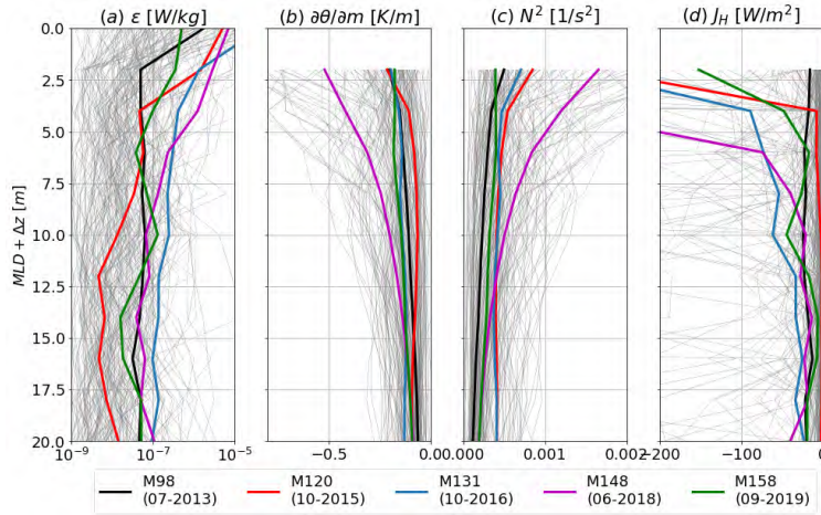
Fig. 2: (a) Turbulent dissipation ( \epsilon ), (b) temperature gradient, (c) buoyancy frequency and (d) turbulent heat flux as a function of depth below mixed layer. Colored lines give the mean for each cruise. Grey lines show the averages of each microstructure station.
