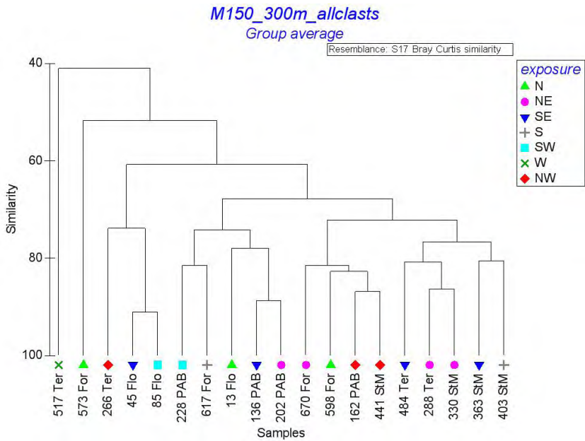
Fig. 1: Cluster analysis of sediments from all 300m Stations of M150 Cruise concerning the entire component spectrum (bioclasts, relictic material, lithoclasts). Ter = Terceira, Flo = Flores, StM = St. Maria, For = Formigas, PAB = Princess Alice Bank.
