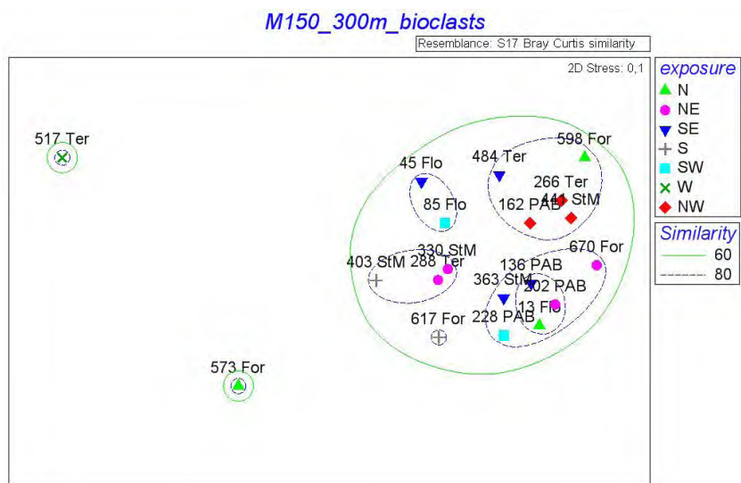
Fig. 2: nMDS plot of sediments from all 300m Stations of M150 Cruise concerning the entire bioclcasts component spectrum. Ter = Terceira, Flo = Flores, StM = St. Maria, For = Formigas, PAB = Princess Alice Bank.
