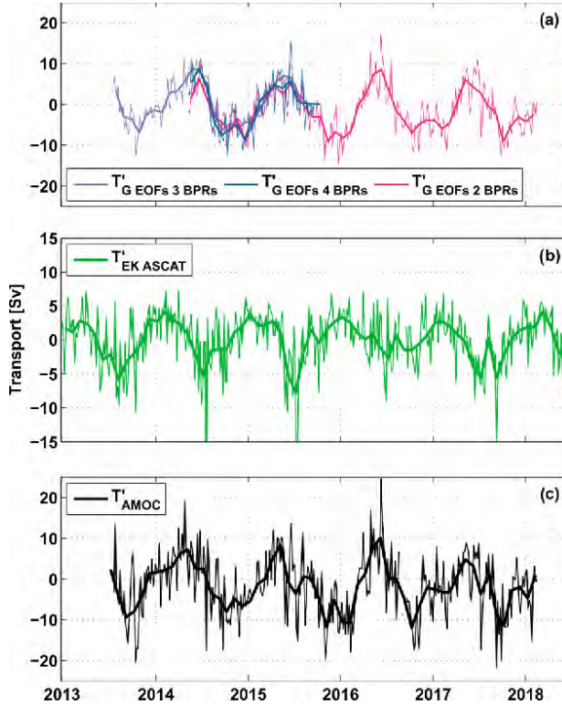
Fig. 2: Anomaly time series at 11° S of (a) the upper-ocean geostrophic transport derived from bottom pressure recorder (BPR) and altimetric sea level measurements, (b) the Ekman transport derived from ASCAT wind stress, and (c) the resulting AMOC anomaly transport. Thin lines represent daily values in (a) and 5-daily values in (b, c), bold curves represent monthly averages. Different colors in (a) indicate transport calculations for different sets of bottom pressure records (BPR) – 4 BPRs (petrol), 3 BPRs (purple) and 2 BPRs (magenta) (from Herrford et al., 2021).
