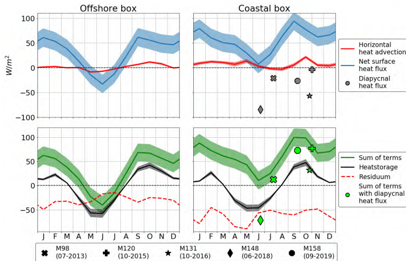
Fig. 3: (a) & (b) Climatology of terms of the mixed layer heat budget in \text{W/m}^2 . Blue line shows the net surface heat fluxes. Red lines show the total horizontal heat advection. Grey markers display the mean heat loss due to diapycnal mixing averaged between 4 and 14m below the mixed layer measured during five cruises (see legend). (c) & (d) Green lines displays the sum of terms depicted in (a) & (b). Black lines show the heat storage term. The residuum between the sum of terms and the heat storage term is shown in red dashed lines. Green marker shows the climatological sum of terms including the measured diapycnal heat fluxes. (a) & (c) shows the spatial average over the offshore box, (b) & (d) shows the spatial average over the coastal box.
