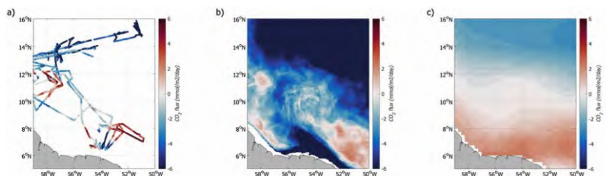
Fig. 2: a) Air-sea \text{CO}_2 flux measured in Jan-Feb 2020 during the EUREC4A-OA/ATOMIC cruise. b) Air-sea \text{CO}_2 flux reconstructed over February 2020. c) February climatology of the air-sea \text{CO}_2 flux over 1998-2015.
