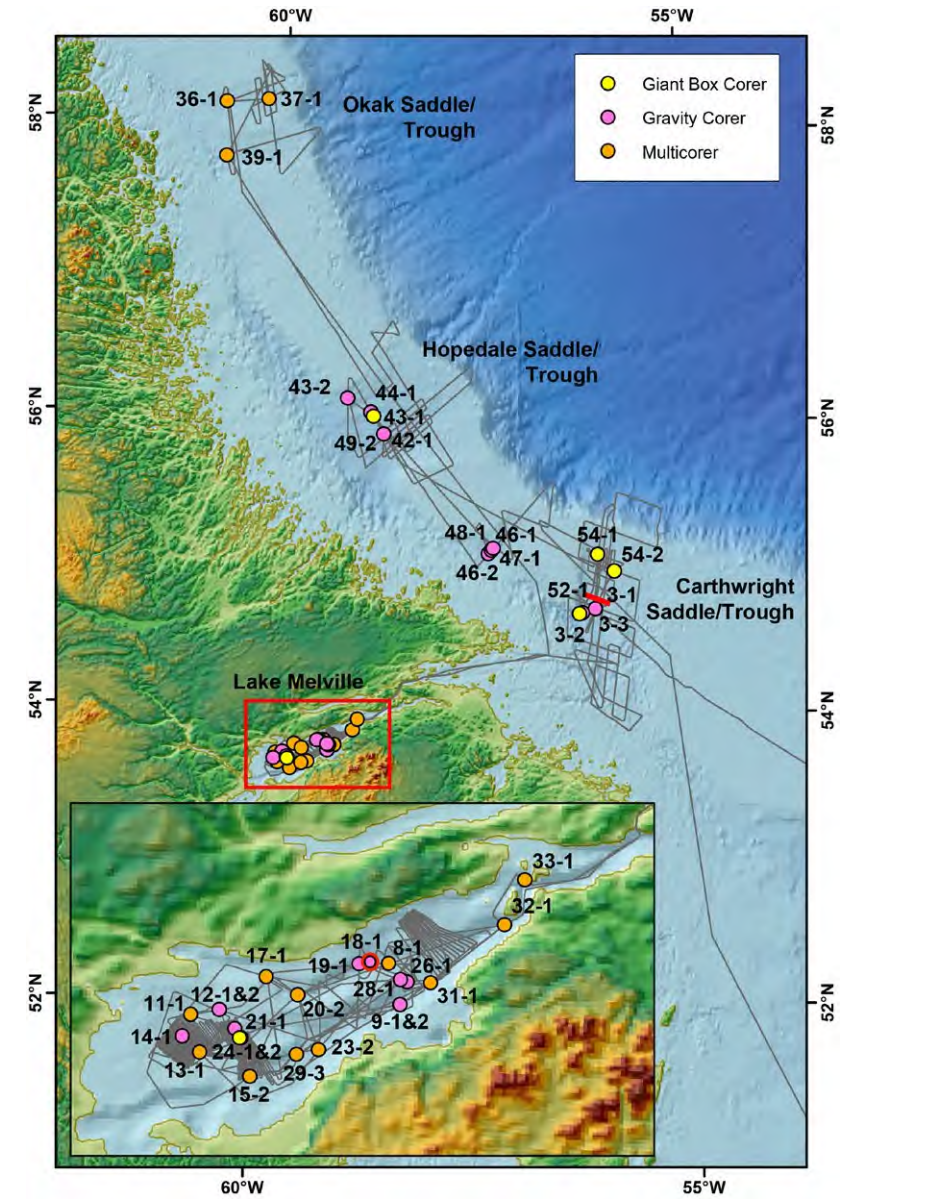
Fig. 1: Research area with location of sediment cores and tracklines of Parasound and bathymetry. Seismic profiles were gathered in the trough systems of the Labrador Shelf. Core MSM84_18-1 shown in Fig. 2 and profile 707 displayed in Fig. 3 are marked in red.
