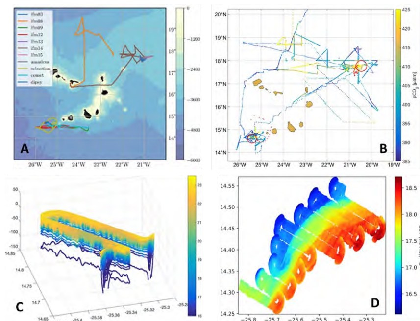
Fig. 3: Examples of deployments of autonomous or airborne instruments for high-resolution observations: (A) Tracks of all deployments of the 11 gliders used during M160, (B) Map of surface p\text{CO}_2 as measured by RV METEOR, 2 Saildrones, and 2 Wave Gliders during M160, (C) 3D visualization of temperature measurements performed by the Towed Instrument Array system (TIA) during M160 on 13/12/2019, and (D) composite map of sea surface temperature from a flight of the Stemme on 12/12/2019 at the southeastern edge of the mesoscale eddy that was located to the southwest of the island of Fogo.
