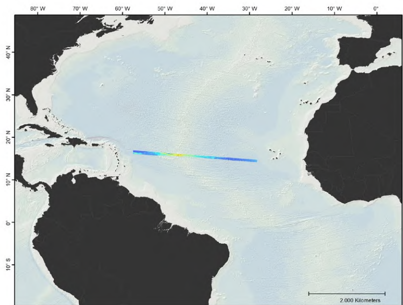
Fig. 1: Overview of the work area showing high resolution bathymetry data obtained during MSM88. GEBCO digital map in the background.
