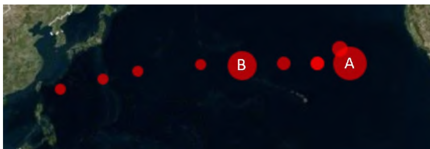
Fig. 2: Comparison of concentrations of surface floating plastic particles. A – Great Pacific Garbage Patch, B – Papahānaumokuākea Marine National Monument
